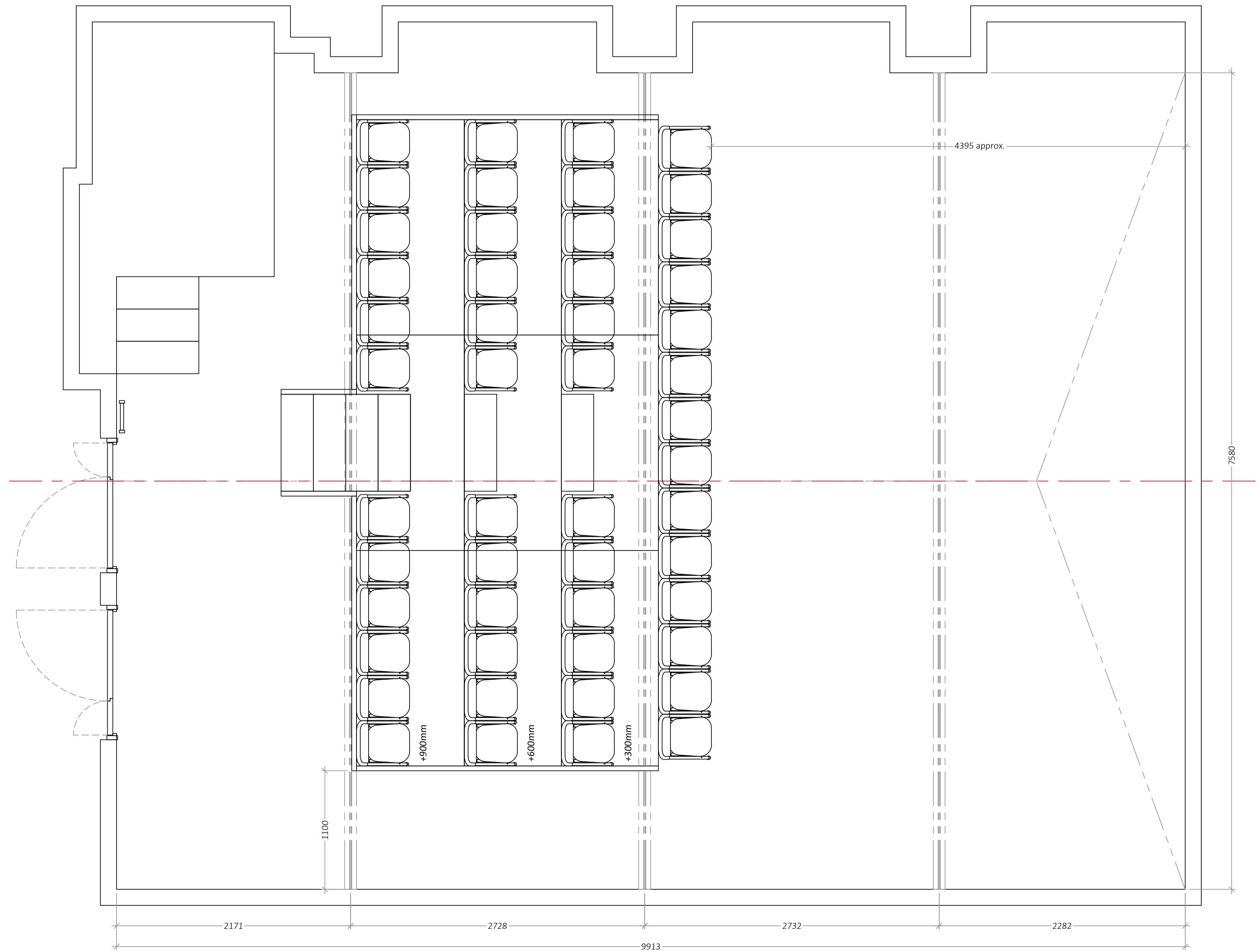
GROUND PLAN Scale 1:25
